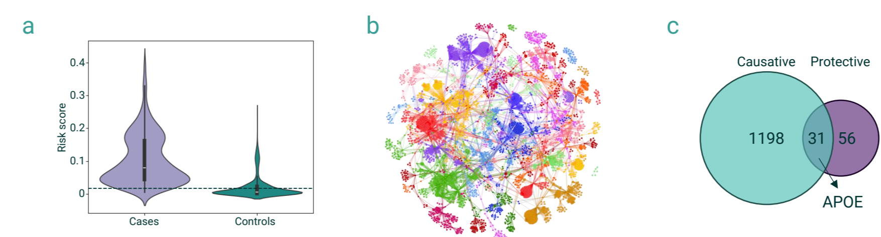
Figure 5. (a) Violin plot showing the distribution of risk scores for AD cases and controls in the ROSMAP/MSBB/Mayo dataset. The dashed line shows the risk score threshold selected to identify the actively protective cohort. (b) Disease architecture diagram demonstrating the 47 communities of SNPs comprising the structure of the Alzheimer's disease patient subpopulations generated by the PrecisionLife platform. Each circle represents a disease-associated SNP genotype, edges represent co-association in patients, and each color a distinct community of SNPs. (c) Venn diagram shows the overlapping genes between the actively protective and causative cohorts from the ROSMAP/MSBB/Mayo cohort.
